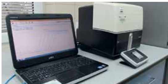
Real-time PCR.
